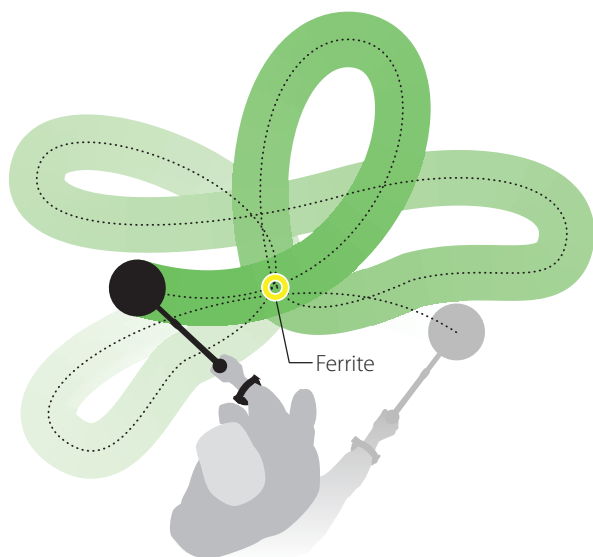
Ground balancing with a ferrite: The sweep path crosses over the ferrite numerous times whilst also covering as much different ground as possible.
